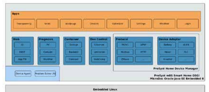
Illustration 3: EnergyBASE architecture
