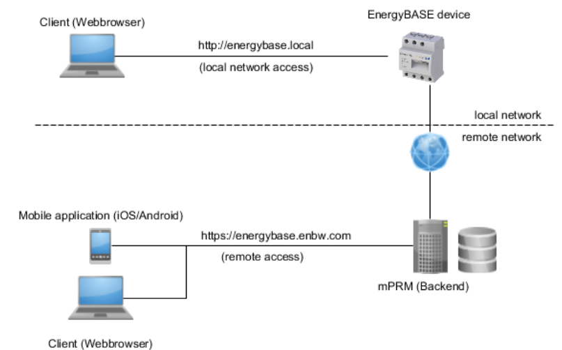
Illustration 2: System components
